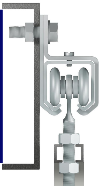
SLIDE-10-WH-30 Galvanised steel 2 Wheel hanger with short 30mm thread
