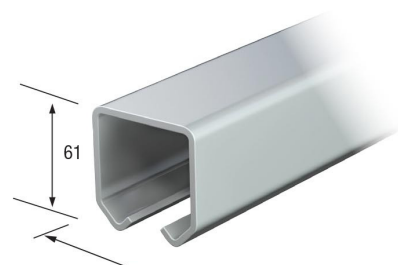
SLIDE-10T-2M SLIDE-10T-3M Galvanised steel Sliding track
