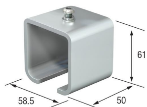
SLIDE-10-DWB-U Galvanised steel U bracket C/W threaded hole, skt screw, washer
