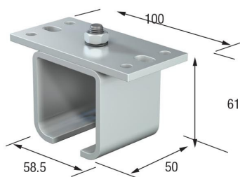
SLIDE-10-WB-S Galvanised steel Single wall bracket - soffit fix
