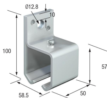
SLIDE-10-WB-F Galvanised steel Single wall bracket - face fix
